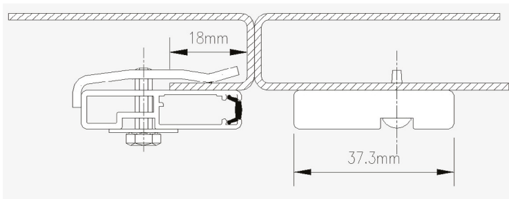
Fig 1: 743 000 Fixing Clamp and Self-Tapping Screw
