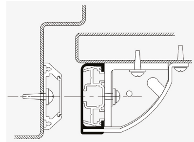
Fig 2: 744 020 Self-Tapping Screw and standard fixing
